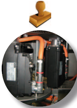
Motors with servo drive on board on the carousel labeling machine
