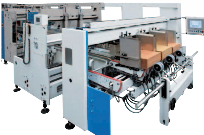
Machine for erecting carton blanks
